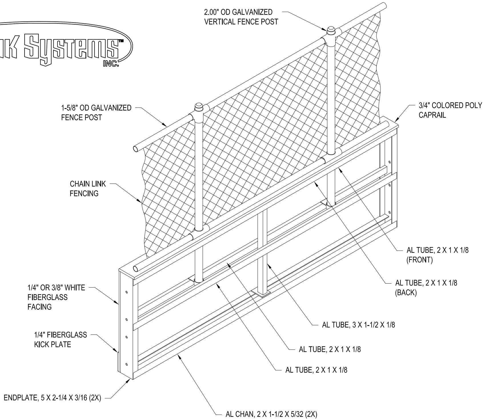
LEGACY PRO - ALUMINUM POSTED W/FENCE
